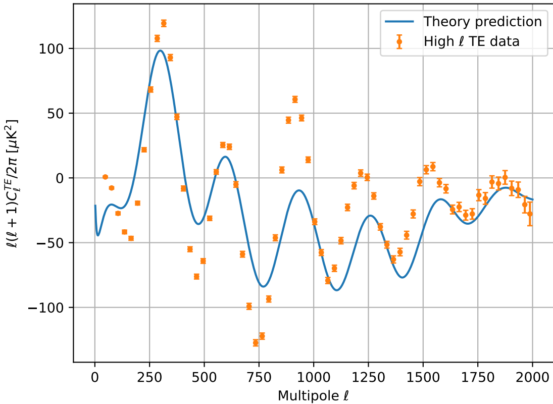
The temperature-polarization cross power-spectrum
